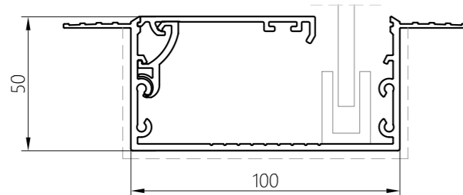
HEM BAR BOX S100x50SS (OPTIONAL)
