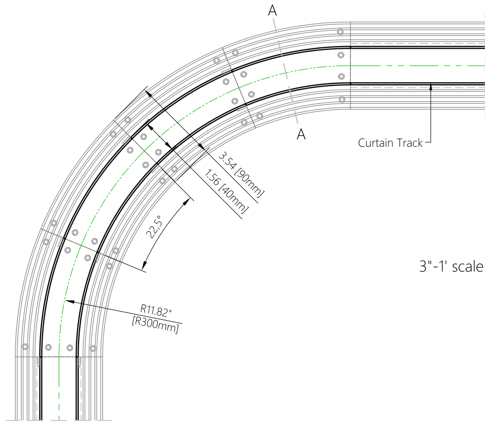
TRACK CURVE SECTION R300
