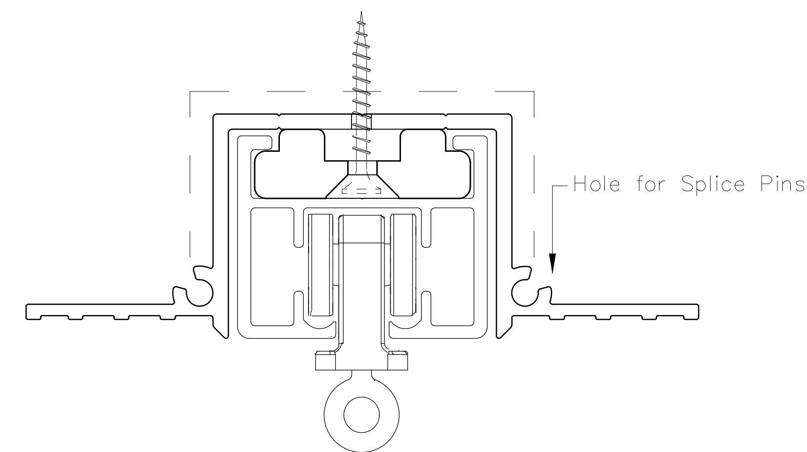
SECTION A-A TT2F PROFILE (OPTIONAL)
